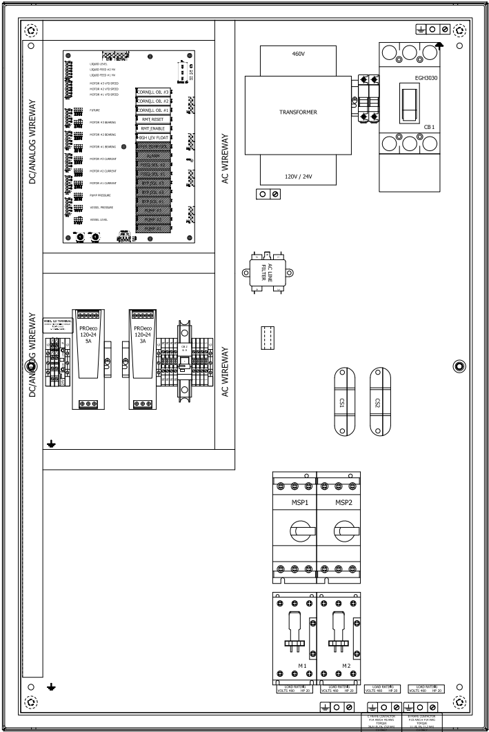
SUBPLATE VIEW CARBON STEEL, PAINTED WHITE 34.2"(H) X 24.2" (W) WITH EDGE FLANGES
